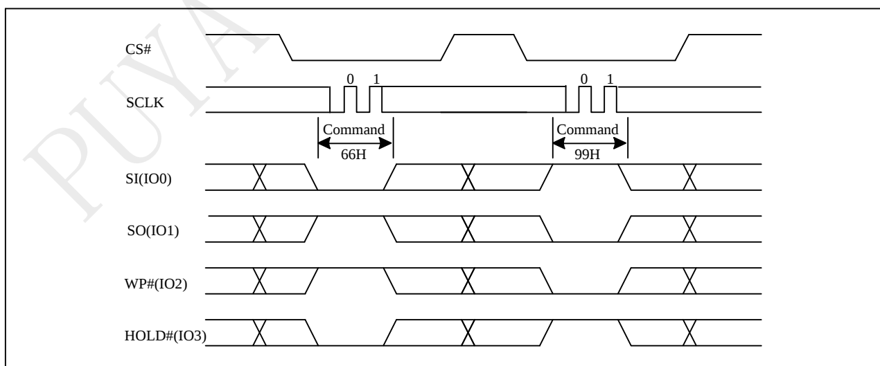
Figure 10-57b Reset Sequence(QPI)
