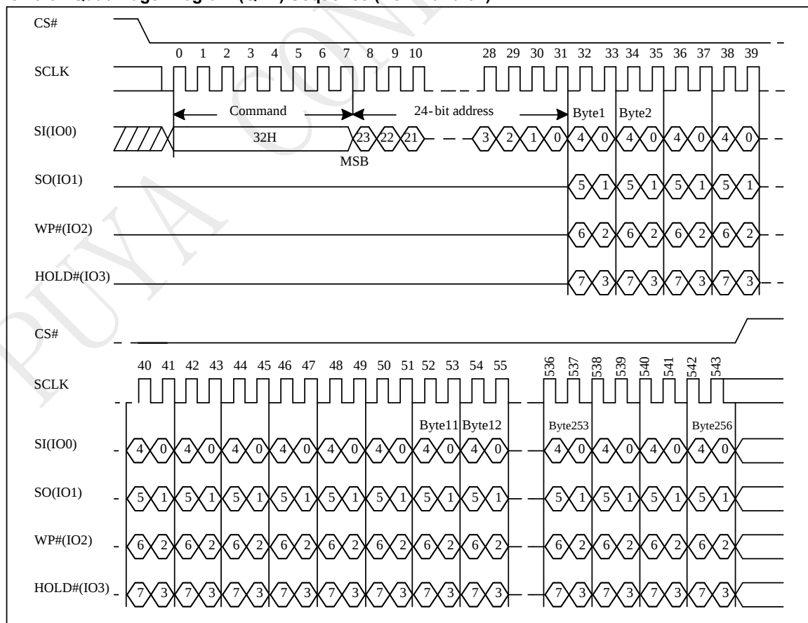
Figure 10-34 Quad Page Program (QPP) Sequence (Command 32)
