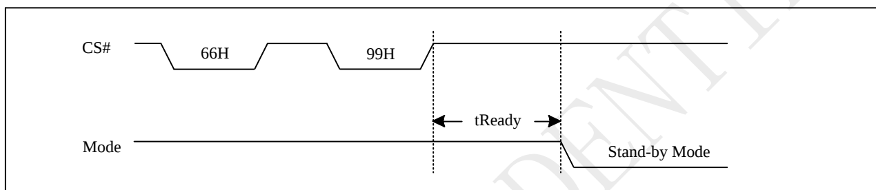
Figure 10-57a Reset Sequence
