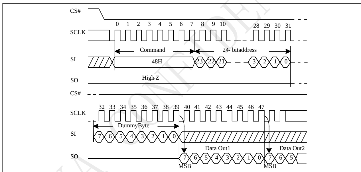
Figure 10-41 Read Security Registers (RDSCUR) Sequence (Command 48)
