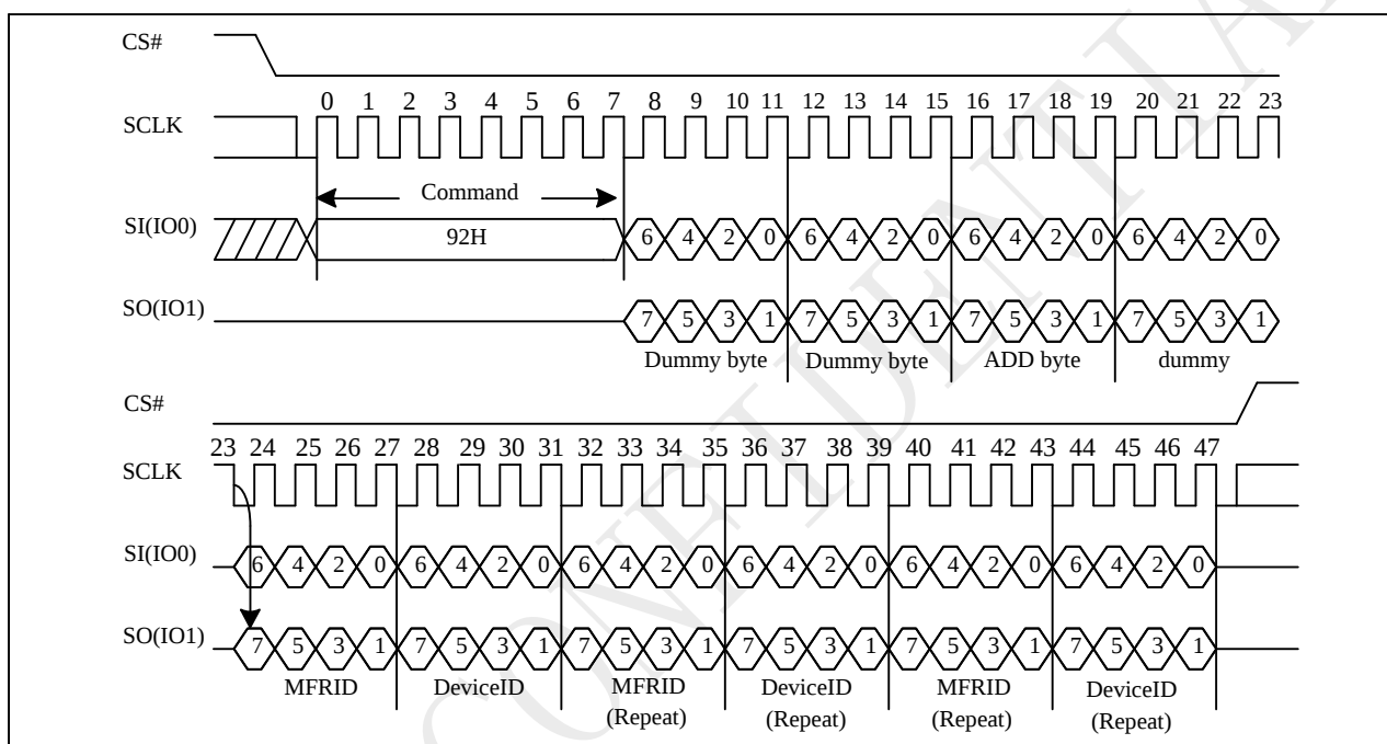
Figure 10-45 DUAL I/O Read Electronic Manufacturer & Device ID (DREMS) Sequence (Command 92)
