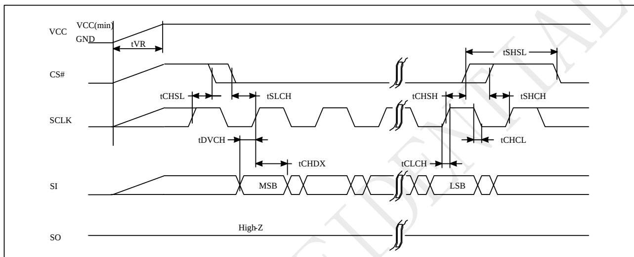
Figure 5-9 Power-up Timing
